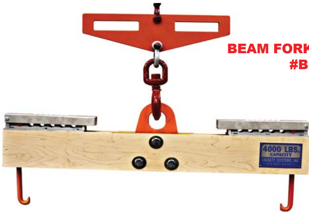
BATTERY LIFTING BEAM #B4000 & #B6000
